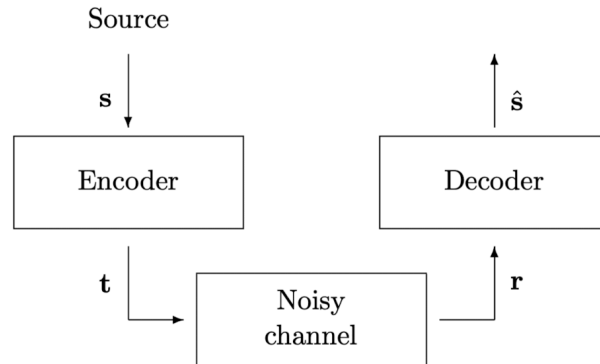
Figure 1: Communication system model
