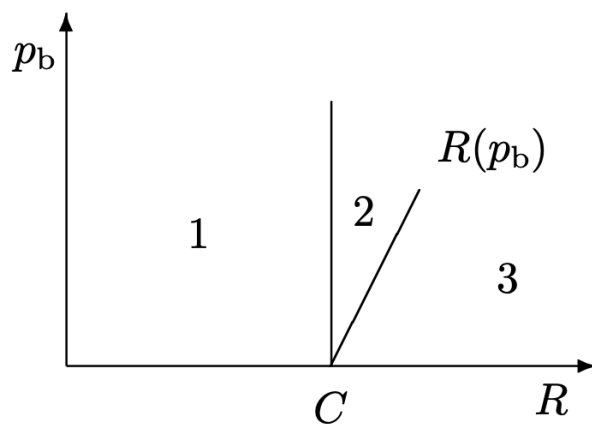
Figure 8: Portion of the R, p_b plane to be proved achievable (1,2) and not achievable (3)
